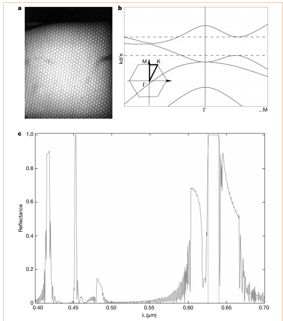
Figure 1 Structure and optical properties of a sea mouse hair from Palm Beach, New South Wales, Australia. a , Electron micrograph of a section of the spine (the dark regions are chitin). b , E , polarization photonic band structure for a hexagonal crystal of voids in chitin, near the four-fold degenerate point on the \Gamma -axis (dashed lines indicate a partial band gap). \Gamma , M and K are the corners of the irreducible part of the first Brillouin zone; k is the free space wavenumber. c , E , polarization total reflectance for normally incident radiation for a hexagonal structure having 500 layers of voids in chitin (dashed lines indicate the partial bandgap of b ). Reflectance measurements using a Zeiss MMS spectrometer confirm a 100% reflectance in the red.
